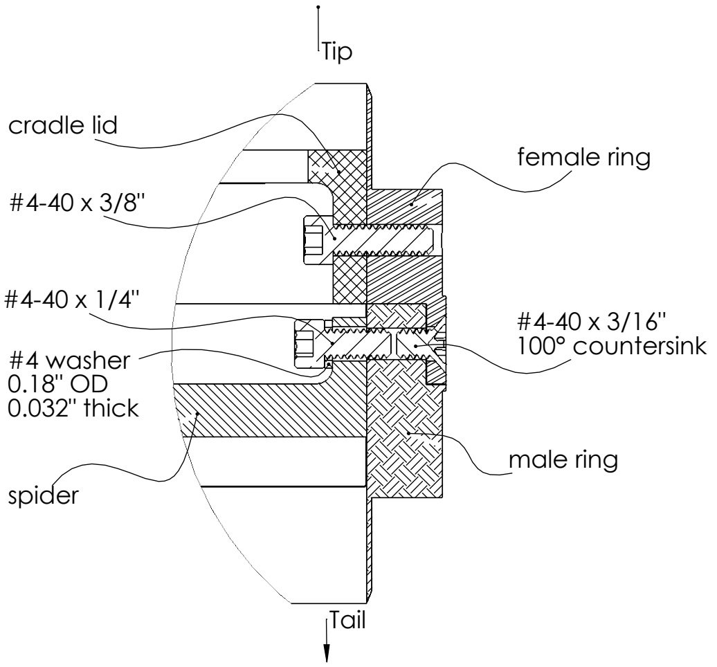
DETAIL B SCALE 2 : 1
